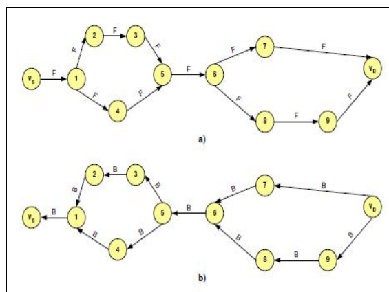
Figure 1: Route Discovery Phase of ACO
